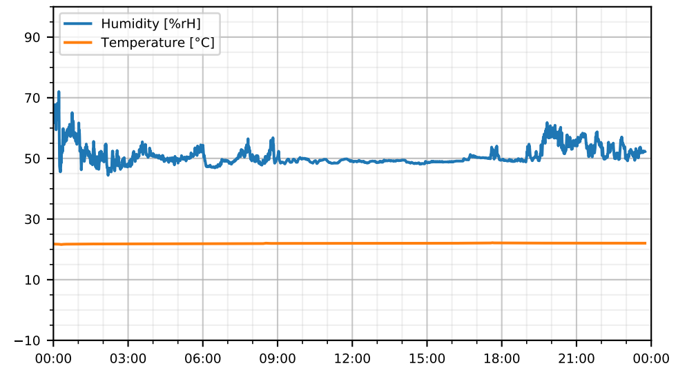
Bathroom
